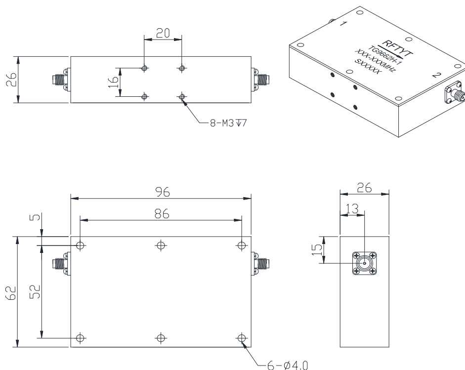
Reverse power 100W type
